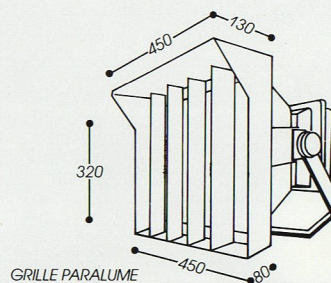
GRILLE PARALUME
